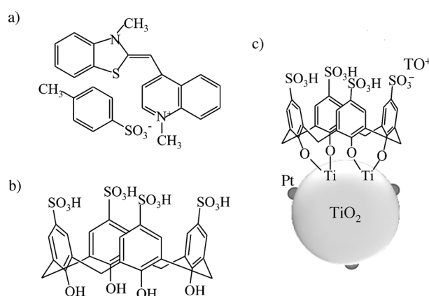
Figure 1. Structures and illustration of a) thiazole orange (TO + ) with p -toluenesulfonate, b) 4-sulfocalix[4]arene (SCA[4]), and c) TO-SCA[4]/Pt-TiO 2 .
